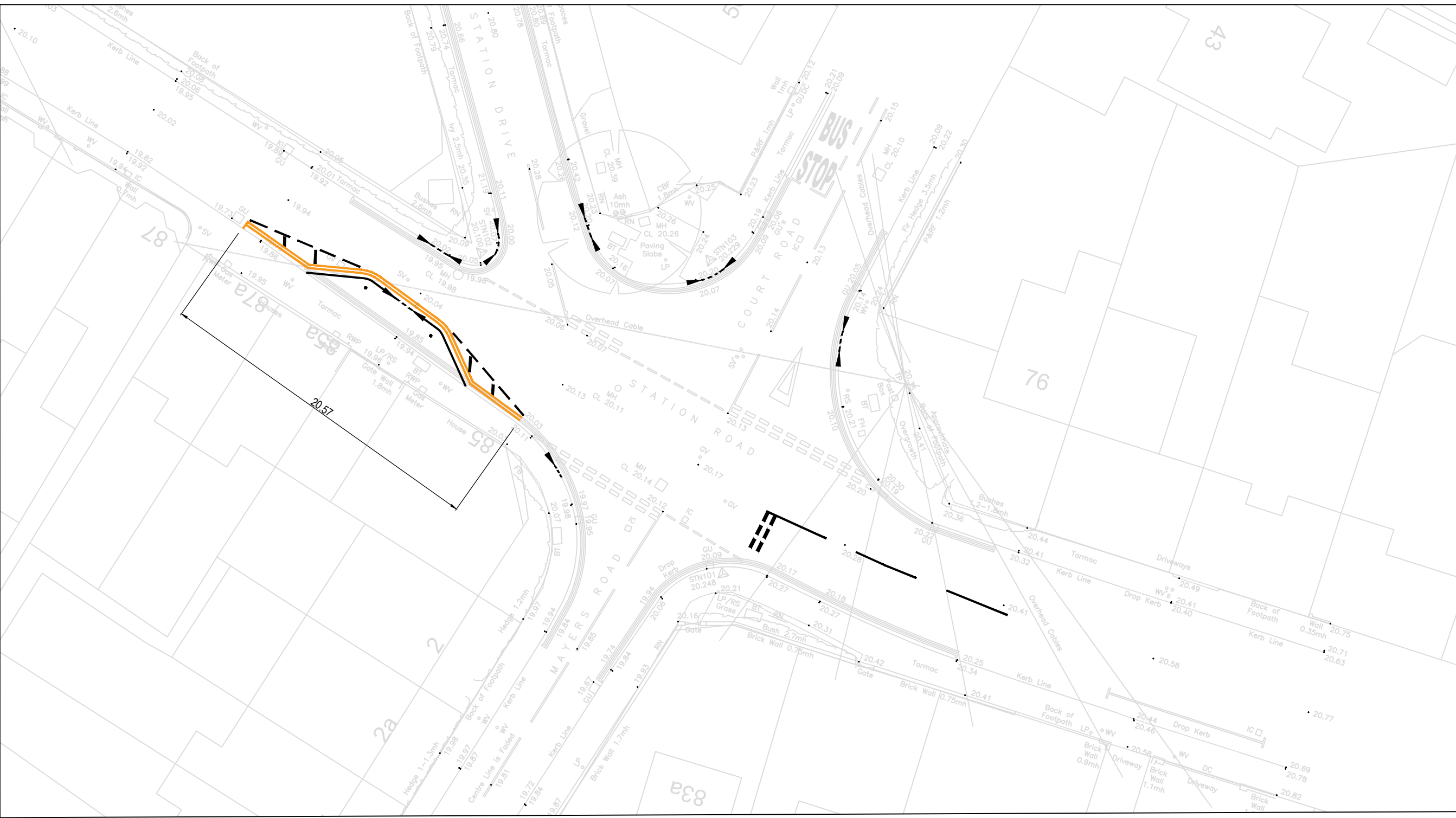
VIEW 2 - PROPOSED DOUBLE YELLOW LINES AT STATION ROAD 1 : 250
